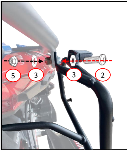
REAR VIEW
